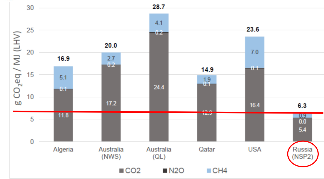
Figure 5-2: Breakdown of overall results, main contributors to GWP – CO 2 , CH 4 and N 2 O (base case)
